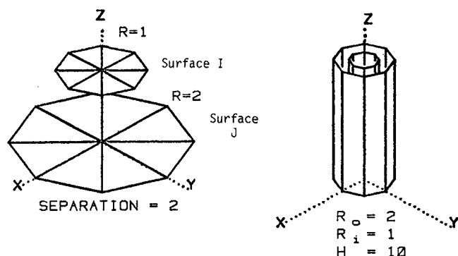
Fig. 5 Radiation between curved surfaces and disks.
