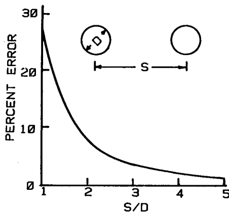
Fig. 7 Error introduced by modeling a cylinder by a rectangle.
